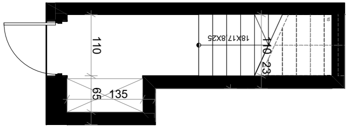
Parter
